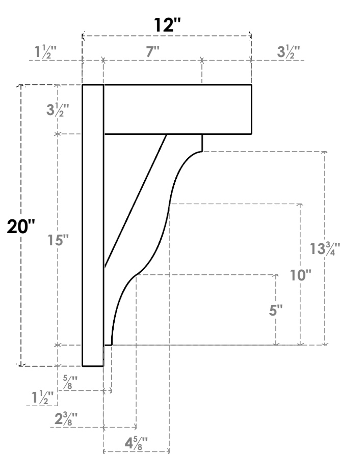
SIDE PROFILE
